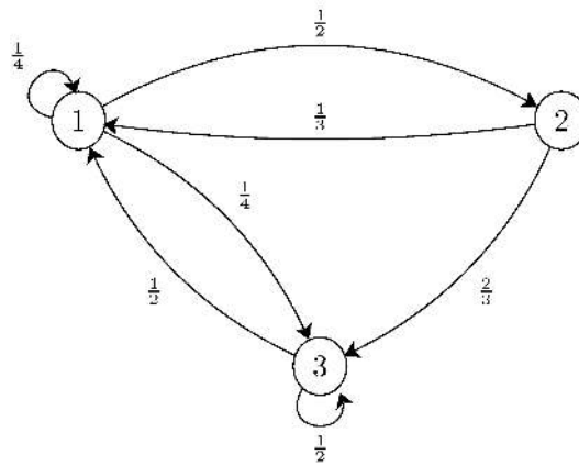
Figure 11.14- A state transition diagram.
