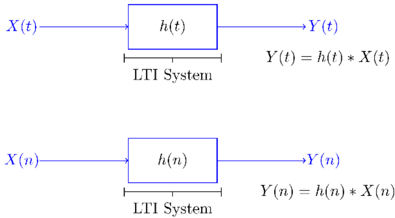
Figure 10.6 - LTI systems.
