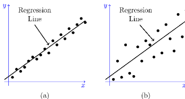
Figure 8.12 - The data in (a) results in a high value of r^2 , while the data shown in (b) results in a low value of r^2 .
