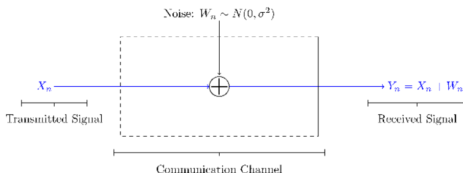
Figure 9.2 - Noisy communication channel in Example 9.2
