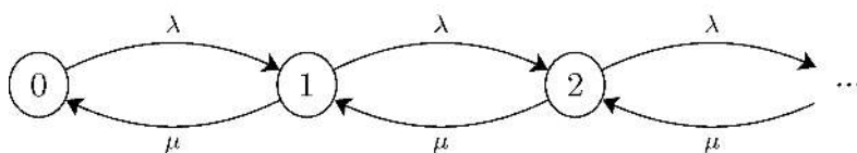
Figure 11.40 - The transition rate diagram for the above queueing system.
